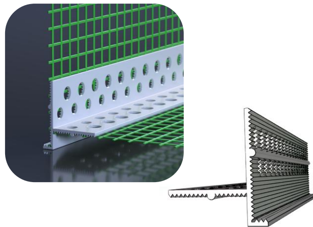
PERFIL PINGADEIRA STANDARD - 2,5M
